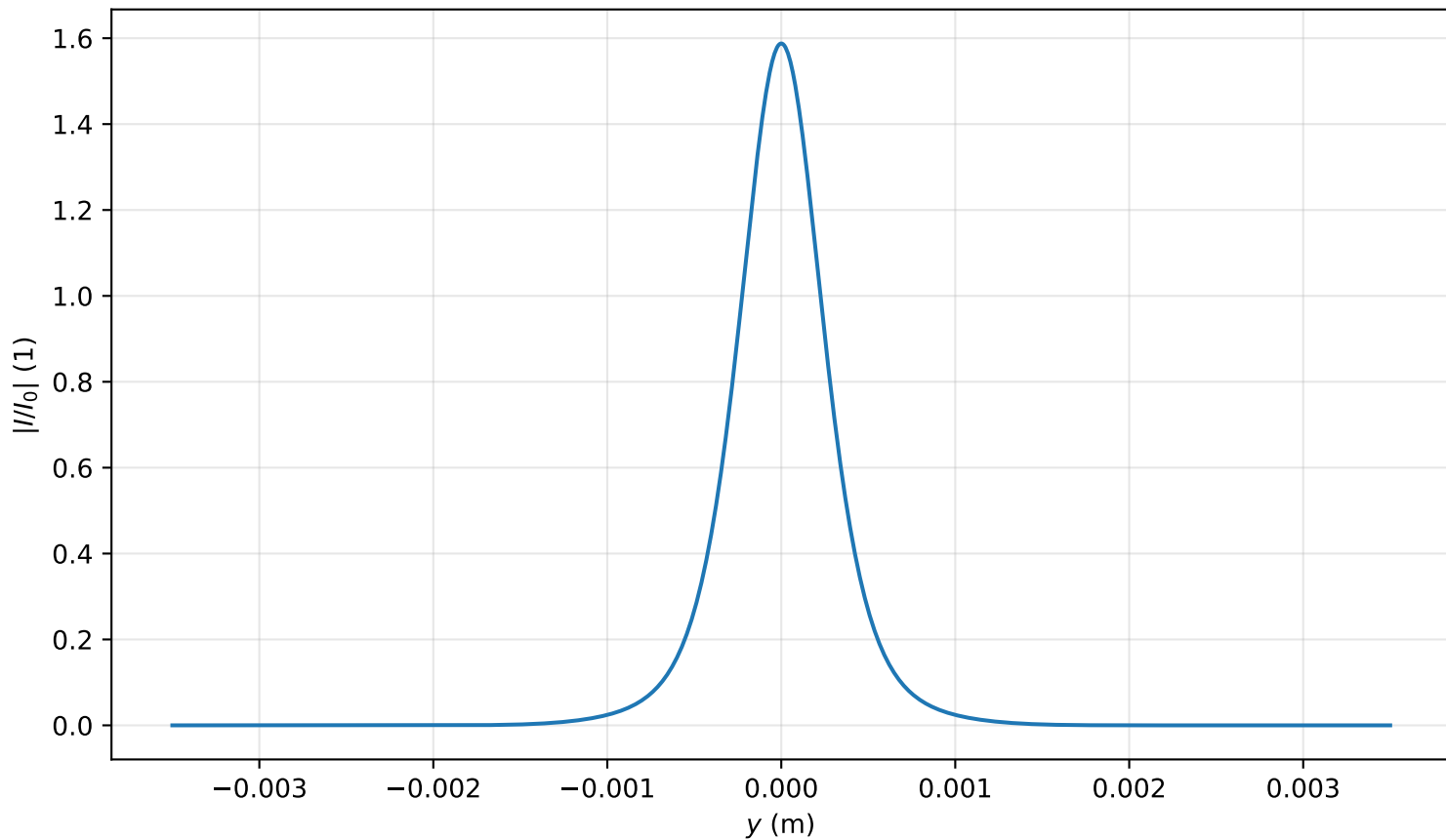
Intensity profile I(x=0, y, z=1.592)/I_0 , P_{in}=0.9P_{cr} , artificial time
